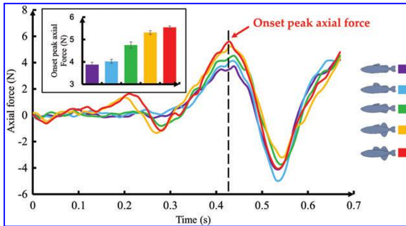
FIG. 7. The measured axial force during the onset stage of linear acceleration (first flapping cycle). Robotic fish body kinematics was programmed as h=0.1 BL, body wavelength = 0.96 BL, and f=1.5 Hz. The inset panel shows the maximum force under different fin states. All of the onset peak axial forces are means from n=5 trials. Error bars are \pm 1 s.e.m. Color images available online at www.liebertpub.com/soro
