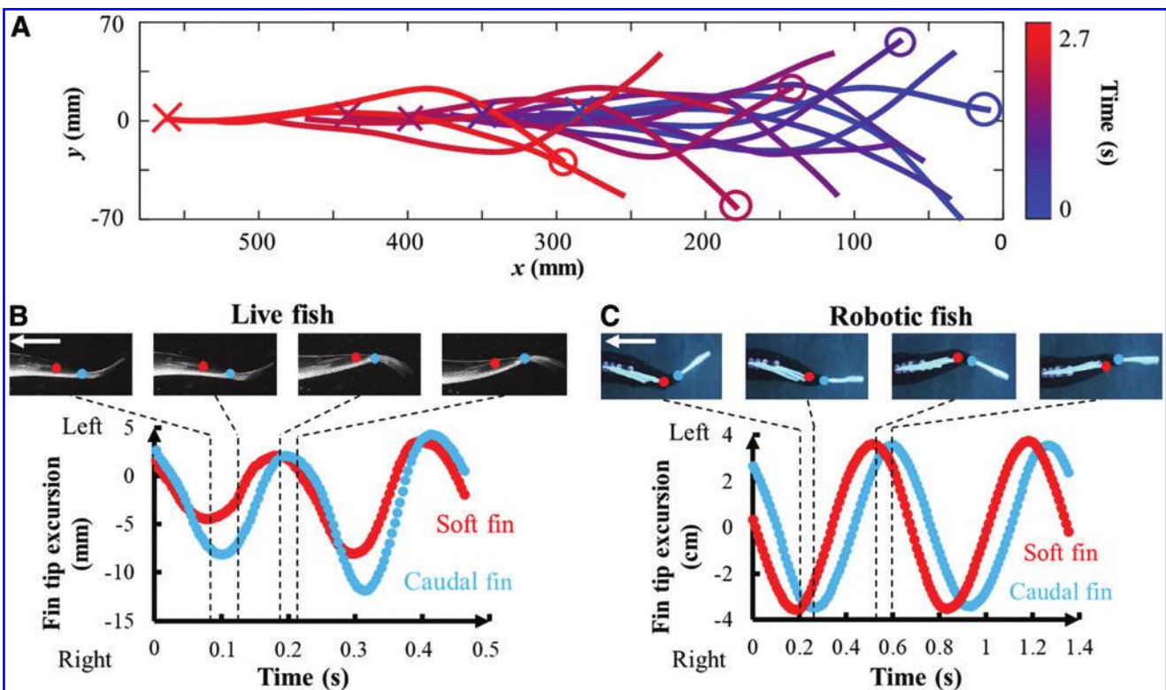
FIG. 5. Kinematics of the robotic fish with median fins. (A) The body midline profiles of the robotic fish extracted from three cycles during linear acceleration ( 0.12 \text{ BL/s}^2 , 0.052 \text{ m/s}^2 ). The snout position is indicated by “x,” and the tail position is indicated by “o.” (B, C) Kinematic patterns for the soft dorsal and tail fins oscillating in tandem during linear acceleration for (B) a live largemouth bass accelerating at 0.17 \text{ BL/s}^2 and (C) the biomimetic robotic fish accelerating at 0.12 \text{ BL/s}^2 , where BL is the fish BL. Panel (C) also includes video images of the two fins moving within a frontal-plane laser sheet over the course of one complete stroke cycle. The red point indicates the trailing edge of the soft dorsal fin and the blue point indicates the leading edge of the caudal fin. Left–right movements of the trailing edges of the soft dorsal fin and the dorsal lobe of the tail are plotted against time for two consecutive flapping cycles in (B) and (C). Color images available online at www.liebertpub.com/soro
